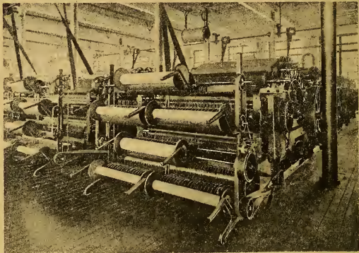
FINISHER WOOLEN CARDING
